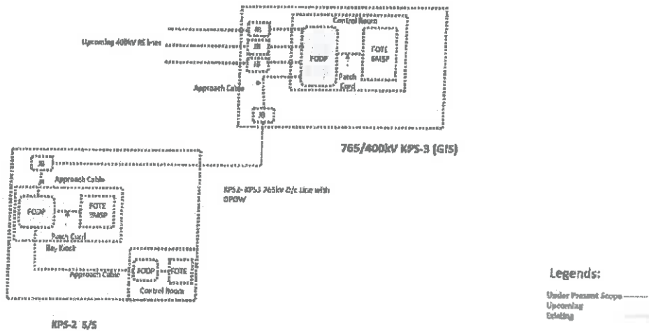
Proposed Communication for Transmission scheme for establishment of 765/400 KV Khavda-3 (KPS-3) in Khavda RE Park
